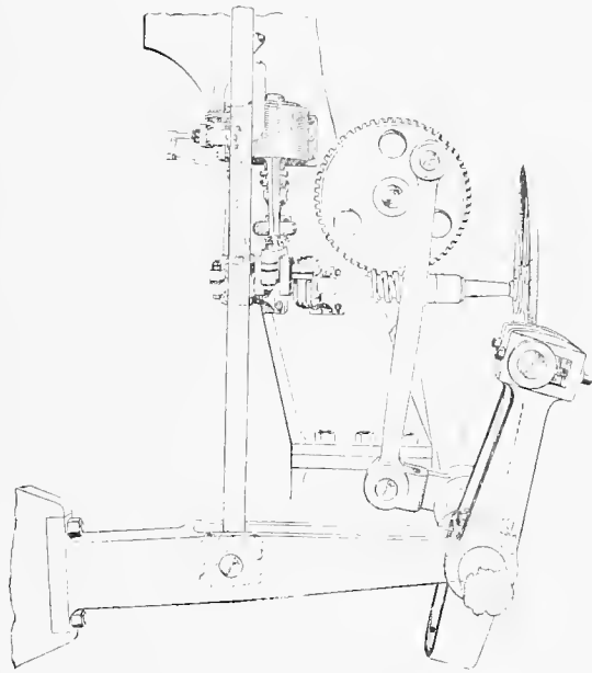
DETAIL OF MARSHALL'S VALVE GEAR.
